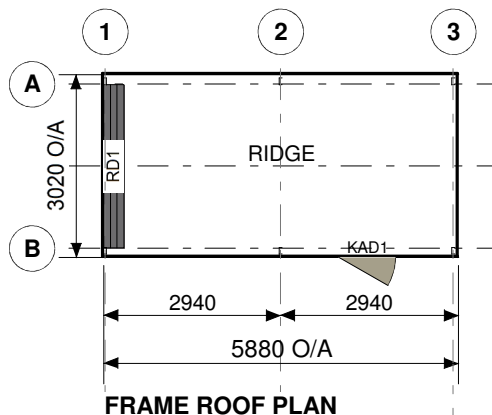
FRAME ROOF PLAN
