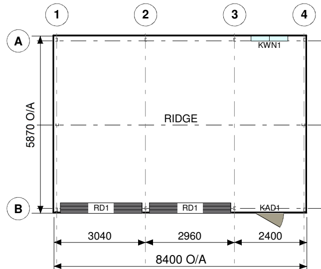
FRAME ROOF PLAN
