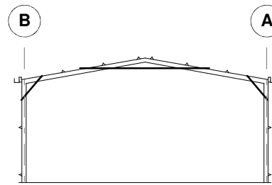
SECTION GRID 2, 3
